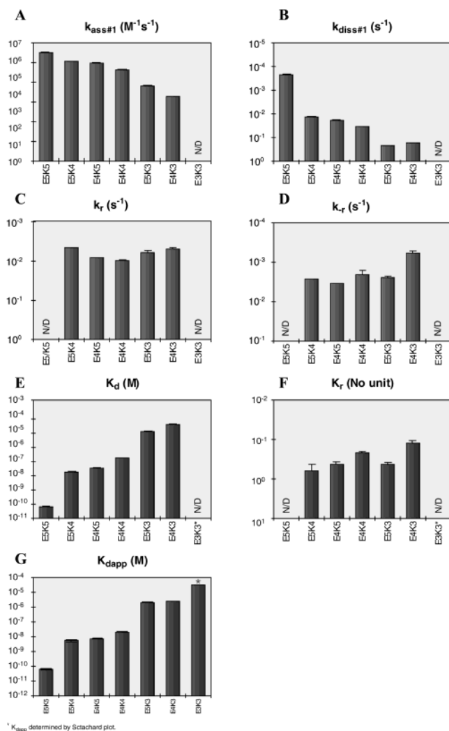
FIGURE 5: The effect of chain length on the kinetic and thermodynamic constants for the E/K interactions derived when using the conformational change (rearrangement) model. Panels A to D: k_{\text{ass}\#1} , k_{\text{diss}\#1} , k_r , and k_r kinetic constants, as determined by globally fitting the different coiled-coil interactions with the conformational change model. Panels E to G: The K_d , K_r , and K_{\text{dapp}} thermodynamic constants that were calculated using the kinetic constants. * K_{\text{dapp}} was determined by Scatchard plot.
